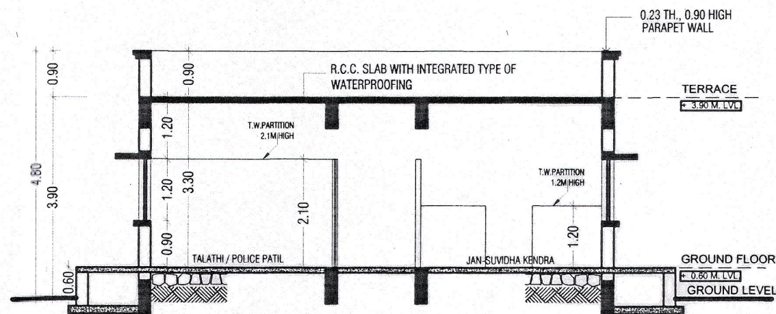
SCHEMATIC SECTION @ A-A
